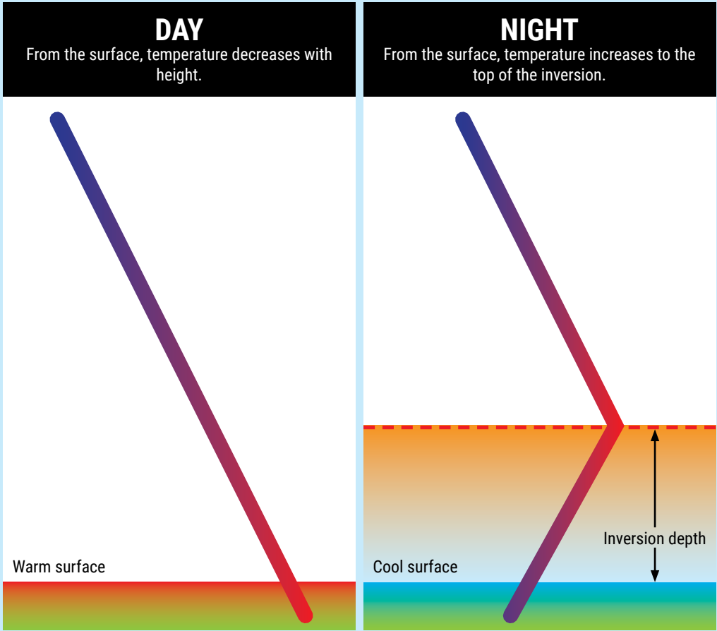
Above: Typical vertical temperature profiles for a point in time during the night and day. The day profile typically cools with height and the night profile typically warms with height to a depth which constitutes the surface temperature inversion layer. The point where the temperature stops increasing is the top of the surface temperature inversion layer.
